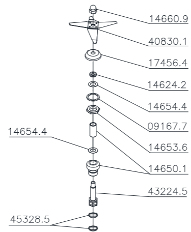
Copo Completo 44651.3
