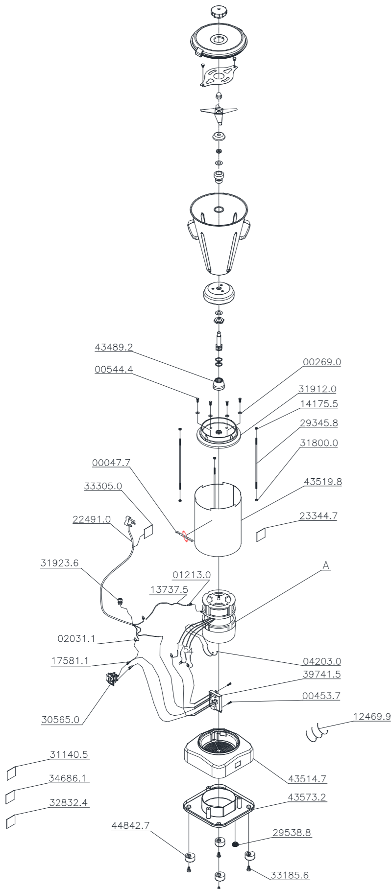
Mancal Completo 43222.9
