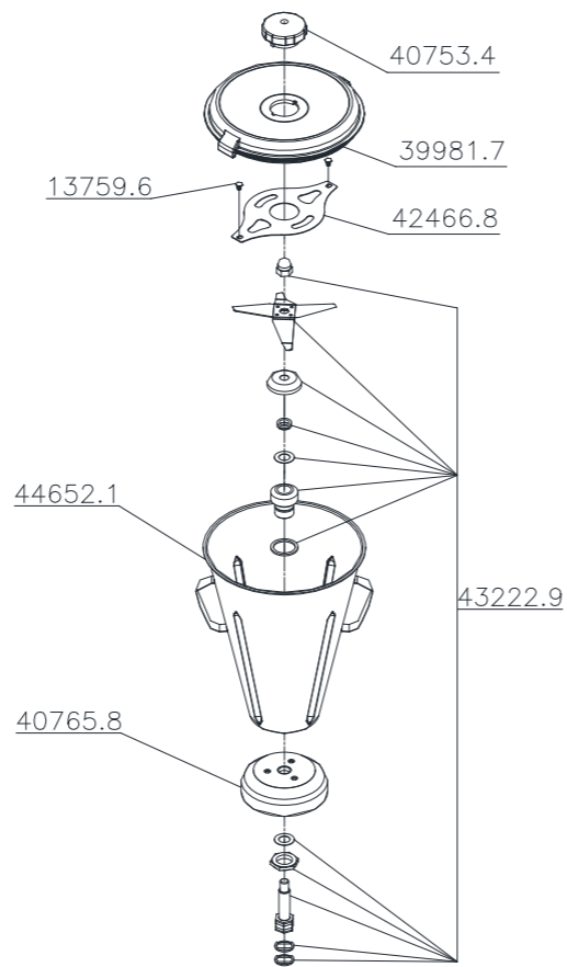
Copo Completo 44651.3
